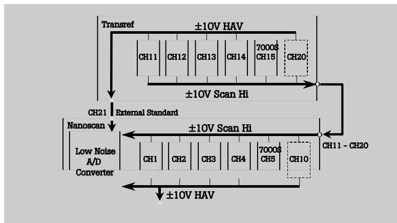
Figure 9 7000 System Analog Bus
