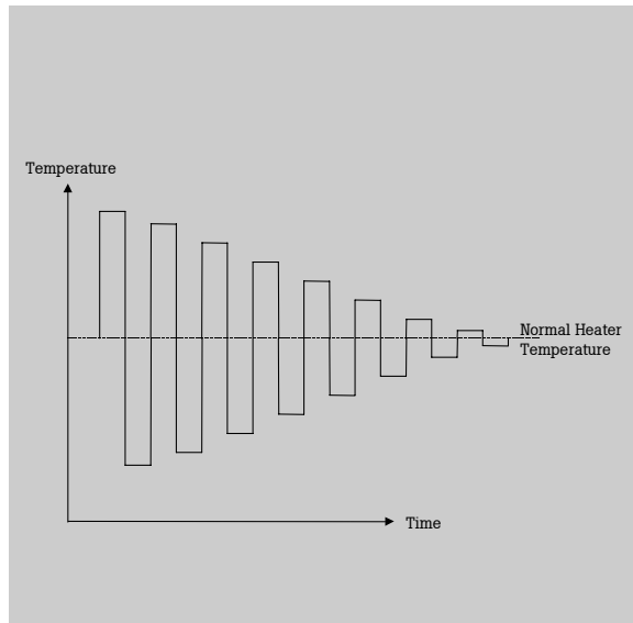
Figure 6 LTZ1000 heater temperature modulation
