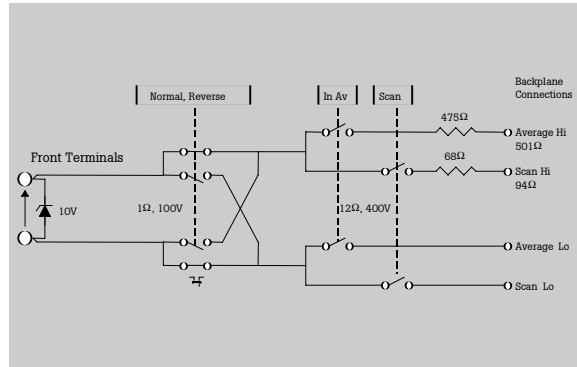
Figure 8 7000 Integral Switching
