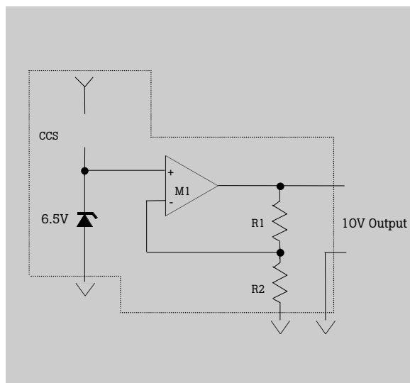
Figure 1 Basic Zener Voltage Reference Standard
