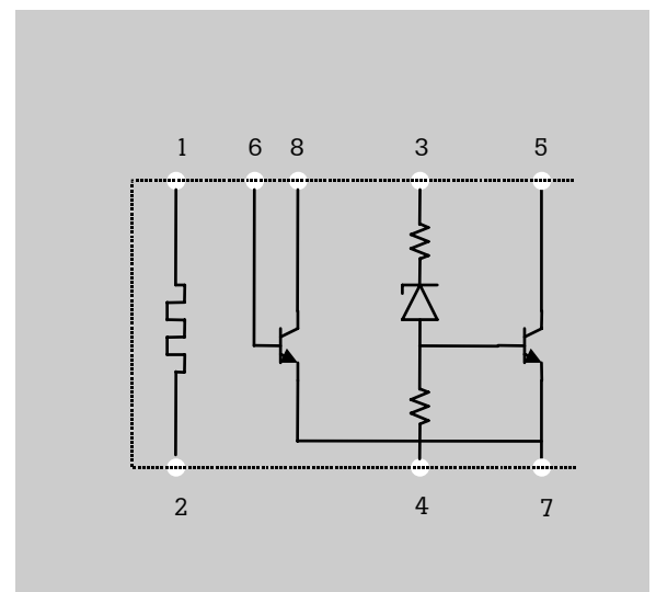
Figure 2 LTZ1000 Schematic
