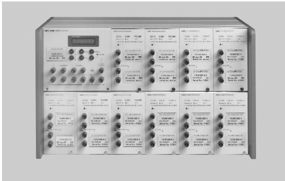
Figure 7 7010N Integrated Volt-Maintenance System
