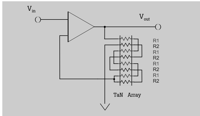
Figure 4 TaN Resistor Array
