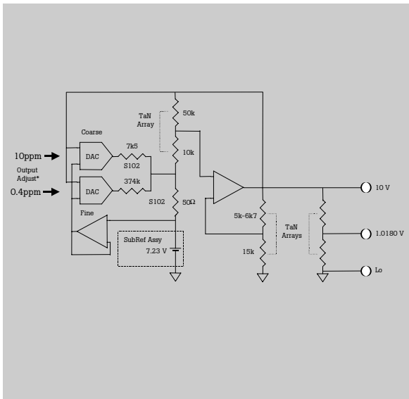
Figure 5 Output Voltage Adjustment of the 7000
